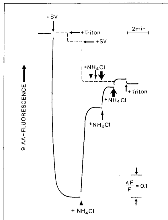
FIGURE 2: Effect of \text{NH}_4\text{Cl} on the transmembrane proton gradient. A total of 200 \mu\text{L} of chromaffin vesicle suspension (2.6 mg of protein/mL of MSPS buffer) was added to 1.8 mL of the same buffer containing 2 \mu\text{M} 9-aminoacridine. \text{NH}_4\text{Cl} (10, 20, or 30 mM final, as indicated by \Delta , thin arrow, or fat arrow) was added from a stock solution of 2 M \text{NH}_4\text{Cl} in MSPS buffer. Triton X-100 was added at a final concentration of 0.1%. In control experiments, the vesicles were first lysed by addition of Triton X-100 (—).
