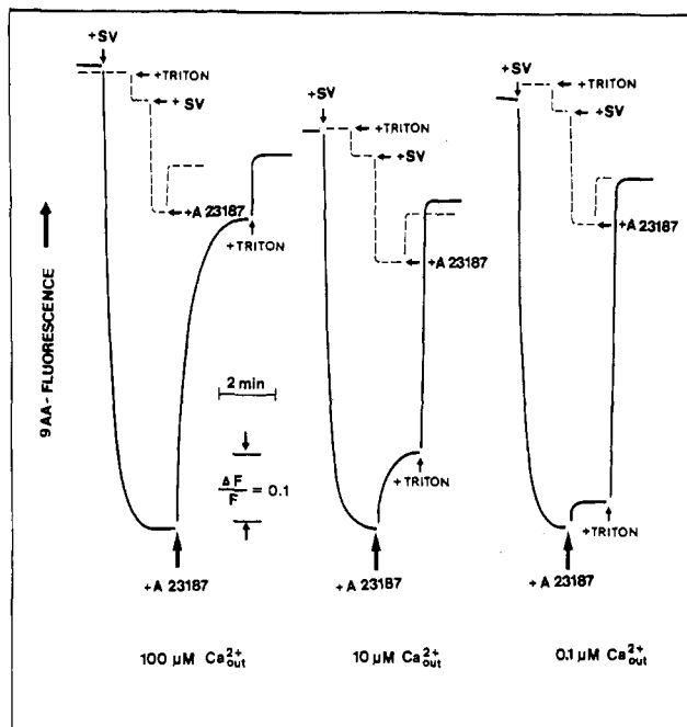
FIGURE 4: A23187-mediated proton transport. Suspensions of secretory vesicles containing 2.6 mg of protein/mL of MSPS buffer (pH 7.3) were incubated with 100, 10, or 0.1 \mu\text{M} free \text{Ca}^{2+} as established by the \text{Ca}^{2+} electrode. A total of 200 \mu\text{L} of these suspensions was added to 1.8 mL of MSPS buffer containing 2 \mu\text{M} 9-AA and identical free \text{Ca}^{2+} concentrations; 5 \mu\text{g} of A23187/mg of protein was used. As a control, the fluorescence of vesicles, lysed with 0.1% of the detergent Triton X-100, was determined under identical conditions (—).
