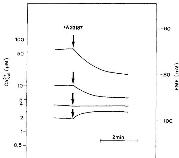
FIGURE 6: A23187-mediated \text{Ca}^{2+} transport in the presence of \text{NH}_4\text{Cl} . Chromaffin vesicles were incubated as described in the legend to Figure 1; 5 \mu\text{g} of A23187/mg of vesicle protein was used. In addition, 30 mM \text{NH}_4\text{Cl} was present in the incubation medium.
