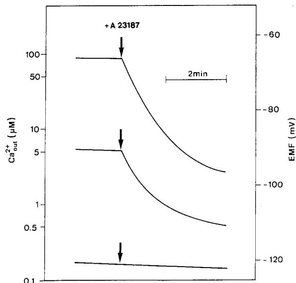
FIGURE 1: A23187-mediated \text{Ca}^{2+} uptake by chromaffin vesicles. The free \text{Ca}^{2+} concentration (the corresponding EMF's are given on the right side) was monitored by a \text{Ca}^{2+} -selective electrode in a suspension of secretory vesicles (1 mg of protein/mL) in MSPS buffer. \text{Ca}^{2+} free was titrated to the desired \text{Ca}^{2+} concentration by addition of small amounts of EGTA or \text{CaCl}_2 . A23187 was added to give a final concentration of 5 \mu\text{g}/\text{mg} of vesicle protein.
