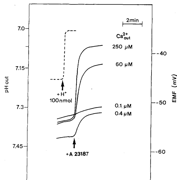
FIGURE 5: A23187-mediated \text{H}^+ release from chromaffin vesicles. Secretory vesicles were resuspended in lightly buffered medium containing 0.5 mM MOPS and sucrose to give a final osmolarity of 420 mosm/kg. \text{Ca}^{2+} free was adjusted by addition of \text{CaCl}_2 or EGTA; 5 \mu\text{g} of A23187/mg of vesicle protein was used. HCl was added for calibration (—).
