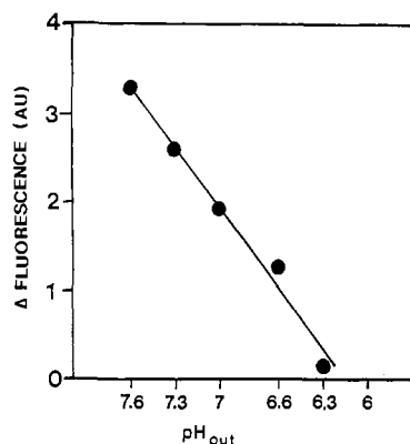
FIGURE 3: Internal pH of isolated secretory vesicles. Chromaffin vesicles were resuspended in 20 mM MOPS or MES and 360 mM sucrose with pH values between 7.6 and 6.3, adjusted with KOH; 200 \mu\text{L} of a vesicle suspension containing 1 mg of protein/mL was added to 2 mL of buffer, with or without \text{NH}_4\text{Cl} (30 mM). The difference in the fluorescence signals after addition of 10 \mu\text{L} of 9-AA (200 \mu\text{M} ) is plotted as a function of the extravesicular pH.
